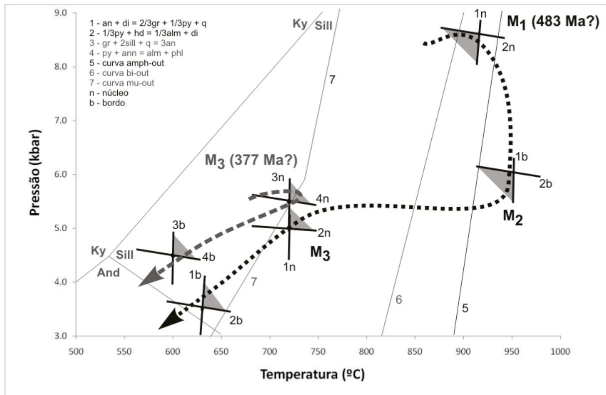
Figure 1 – Summarized P-T-t evolution for the studied samples. In grey is shown the evolution and the most important chemical reactions for the peraluminous rocks, whereas black is for the metaluminous. The dotted line defines the metamorphic evolution for the metaluminous rocks, whereas the dashed line defines the possible metamorphic evolution of the peraluminous rocks. It can be seen that these two rock types, although geographically close presently, had very distinct metamorphic evolutions and were only juxtaposed, probably, during the last metamorphic event ( M_3 ) at 377 Ma ago (Valverde Vaquero et al., 2010). The geothermobarometric estimates for the M_1 and M_2 events are interpreted as maximum T and P, whereas for M_3 they are minimum T and P. Mineral abbreviations are as in Powell et al. (1998). Al_2SiO_5 triple point and muscovite (7) and biotite (6) dehydration-melting curves are as in Spear et al. (1999), whereas amphibole dehydration-melting curve (5) follows Patiño Douce & Beard (1995).
